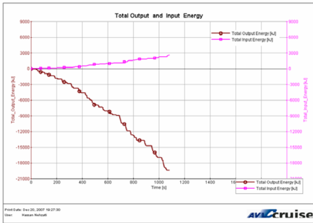
Figure 17: Overall input and output electric energy for for parallel brake strategy
