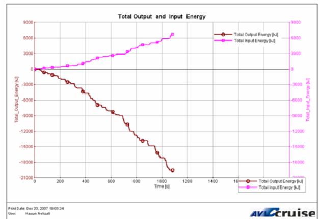
Figure 16: Overall input and output electric energy for optimal energy recovery strategy
