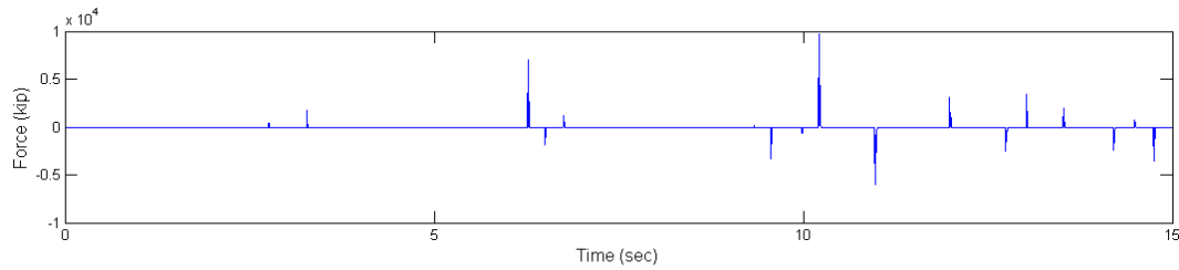
Figure 7. (b) Impact force vs. time, experienced by backwall
