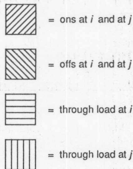
FIGURE 1 Updating with two checkpoints.
