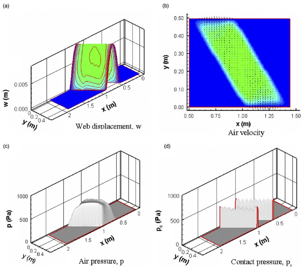
Fig. 5. (a) The web deflection w , (b) airflow vectors, (c) air pressure p and (d) contact pressure p_c at steady state, for Case 1, with \beta = 45^\circ and p_0 = 800 Pa.
