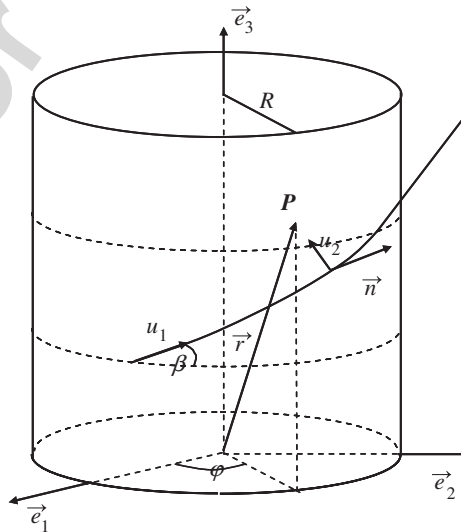
Fig. 3. Coordinates of a point P on Cartesian, \vec{e}_1, \vec{e}_2, \vec{e}_3 , and curvilinear, u_1, u_2, \vec{n} , coordinate systems.
