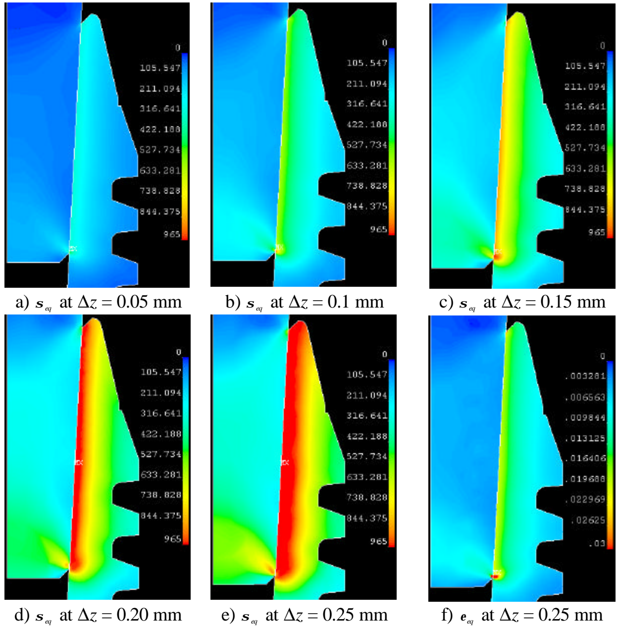
Fig. 7. The von Mises stress distribution for interference depth values of \Delta z = 0.05 - 0.25 mm are given in a)-e). The equivalent von Mises strain for \Delta z = 0.25 mm is given in f). The yield stress for Ti6Al4V ELI is \sigma_Y = 960 MPa, and the ultimate strain is \epsilon_U = 0.08 . Note that the effect of the surrounding bone is included in the analysis but not shown in this figure for clarity of presentation.
