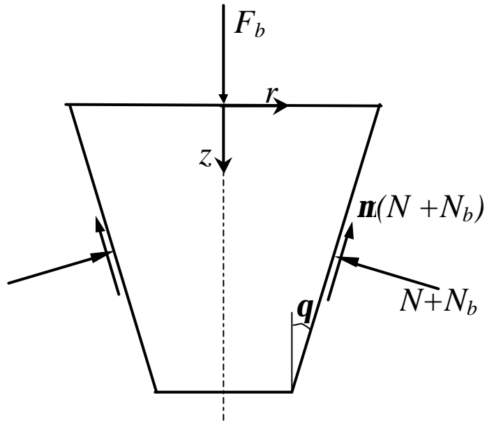
Fig. 2. Equilibrium of the forces acting on the abutment when an axial biting force F_b is applied. A normal force due to initial insertion N , a normal force due to biting N_b , and a tangential force of magnitude m(N+N_b) act on the tapered wall. Note that N and N_b are the resultants of the axisymmetric reaction forces.
