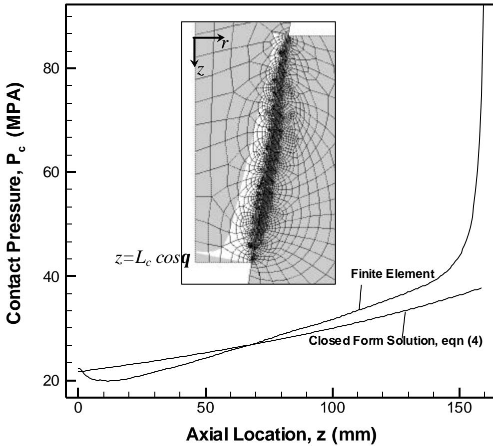
Fig. 5. Comparison of the contact stress distribution predicted by equation (4) and the FEM for q = 9^\circ , L_c/b_1 = 4 , b_2/b_1 = 3 , and d/b_1 = 16 \times 10^{-3} . The insert shows the FE mesh used in the solution and the variation of the contact pressure with respect to the abutment-implant interface.
