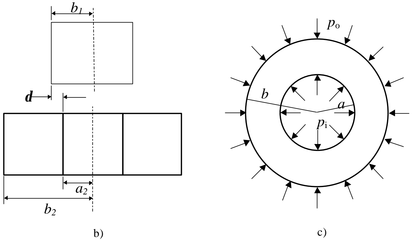
Fig. 3. a) The geometry of a tapered interference fit composed of an outer bone, inner implant and a tapered abutment. b) The geometry of a regular interference fit of a solid shaft with an outer diameter of b_2 and a hollow shaft of outside diameter b_1 and inside diameter a_1 . c) A hollow shaft subjected to inner pressure p_i and outer pressure p_o . The initial interference between the parts in both a) and b) is d .
