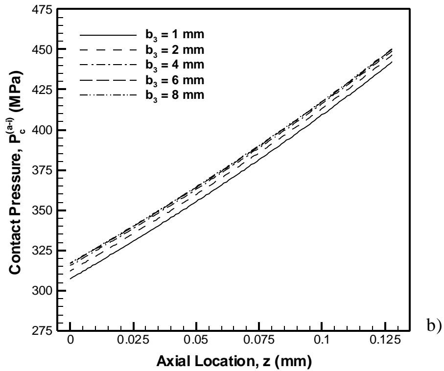
Fig. 6. a) The effect of bone modulus and b) the effect of bone radius surrounding the implant on the contact pressure in the abutment-implant interface P_c^{(a-i)} , calculated by using equation (4).
