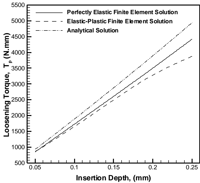
Fig. 9. a) the pull out force and b) the loosening torque for the Bicon implant. The results represent the closed form solution, elastic FEA and elastic-plastic FEA.
