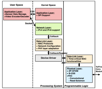
(b) SEANet IoUT software architecture.
