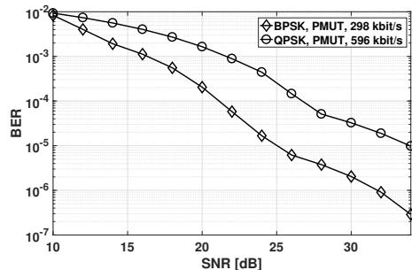
(c) BER versus SNR for different modulation schemes (BPSK and QPSK)
